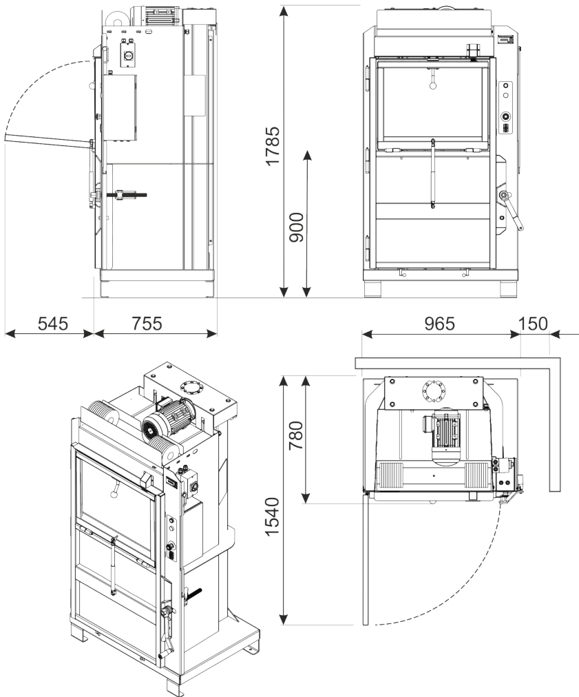
The feed door opens 90° as standard, but can be opened all the way down 180° for customized needs.
