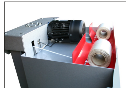
The bale strapping rolls are easily reached at the top. Each roll can be replaced separately.
